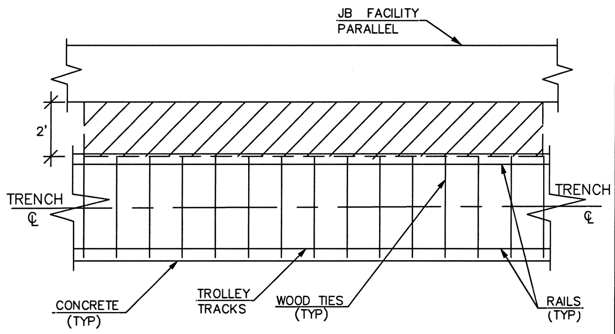
SECTION OF JB FACILITIES PARALLELING TROLLEY TRACKS
