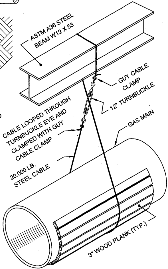
DETAIL "B"
