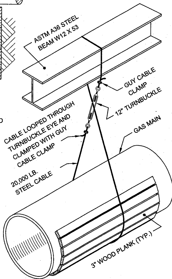
DETAIL "B"
