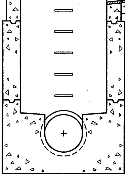
TYPICAL SEWER MANHOLE
