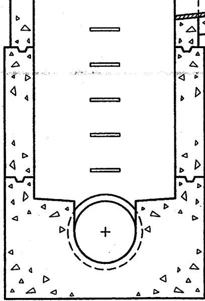
TYPICAL SEWER MANHOLE
