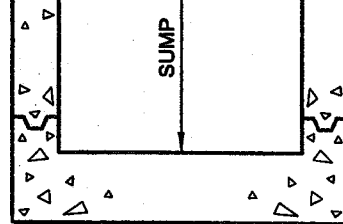
TYPICAL CATCH BASIN
