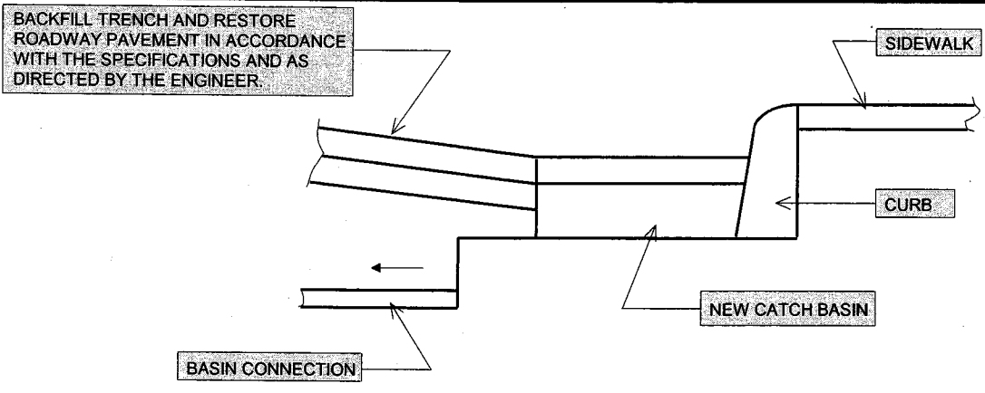
DETAIL - RESTORATION AT BASIN CONNECTION
