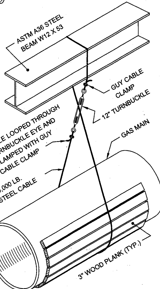
DETAIL "B"
