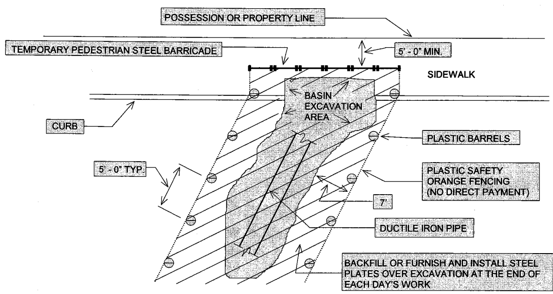
MAINTENANCE OF TRAFFIC FOR CATCH BASIN INSTALLATION FIGURE NO. 1
