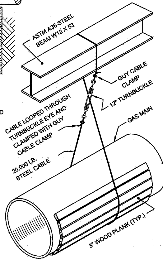
DETAIL "B"
