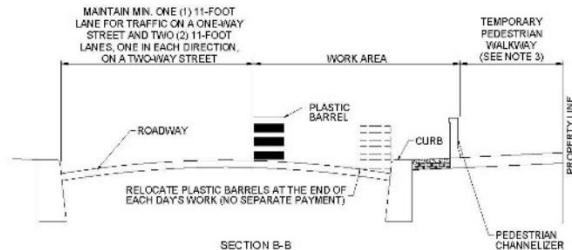
SECTION B-B 410
