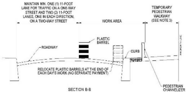
SECTION B-B 1/15
