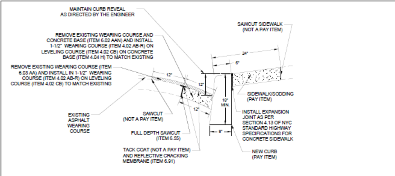
CURB INSTALLATION DETAIL
