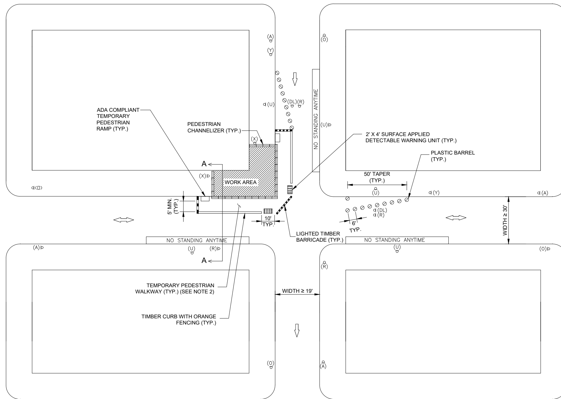
TYPICAL PLAN NOT TO SCALE
