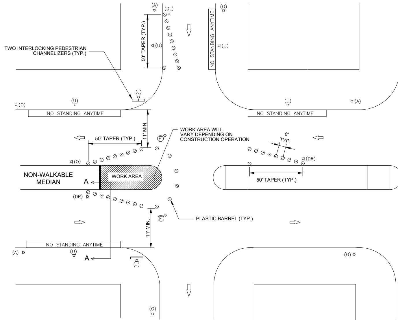
TYPICAL PLAN NOT TO SCALE
