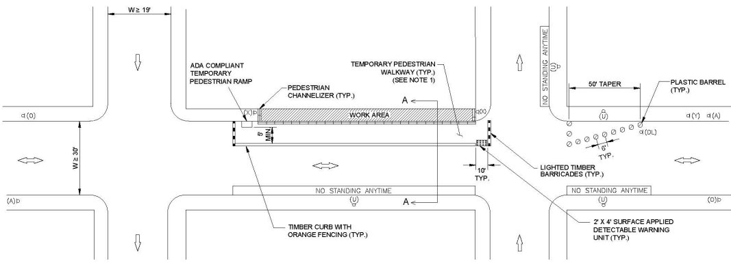
TYPICAL PLAN NOT TO SCALE
