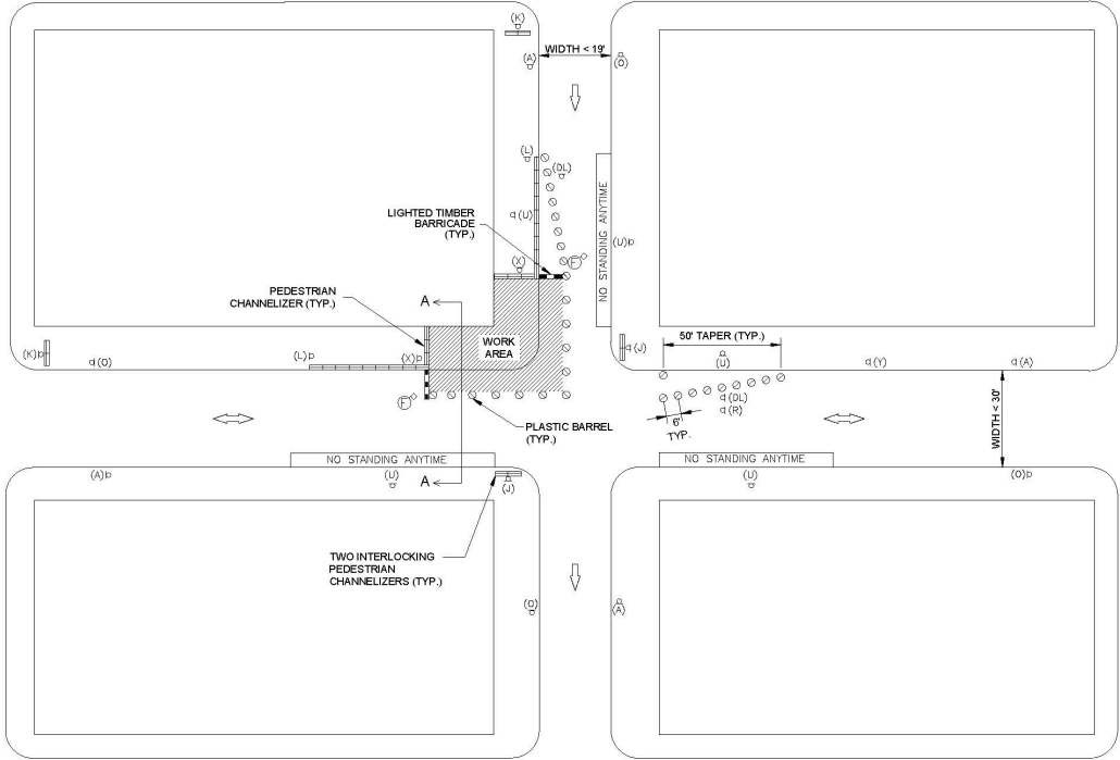
TYPICAL PLAN NOT TO SCALE
