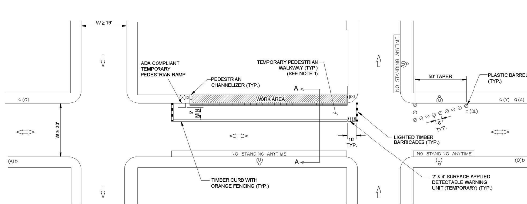
TYPICAL PLAN NOT TO SCALE
