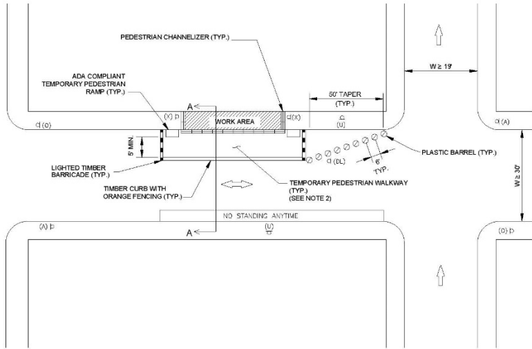
TYPICAL PLAN NOT TO SCALE
