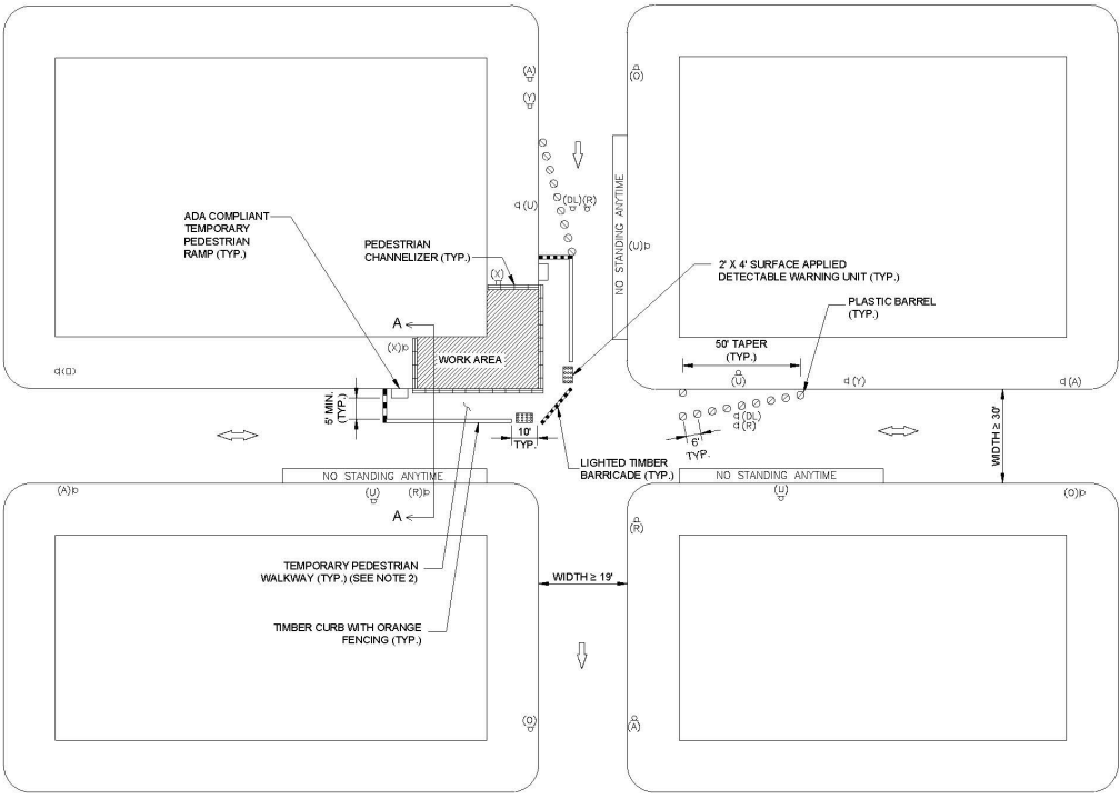
TYPICAL PLAN NOT TO SCALE
