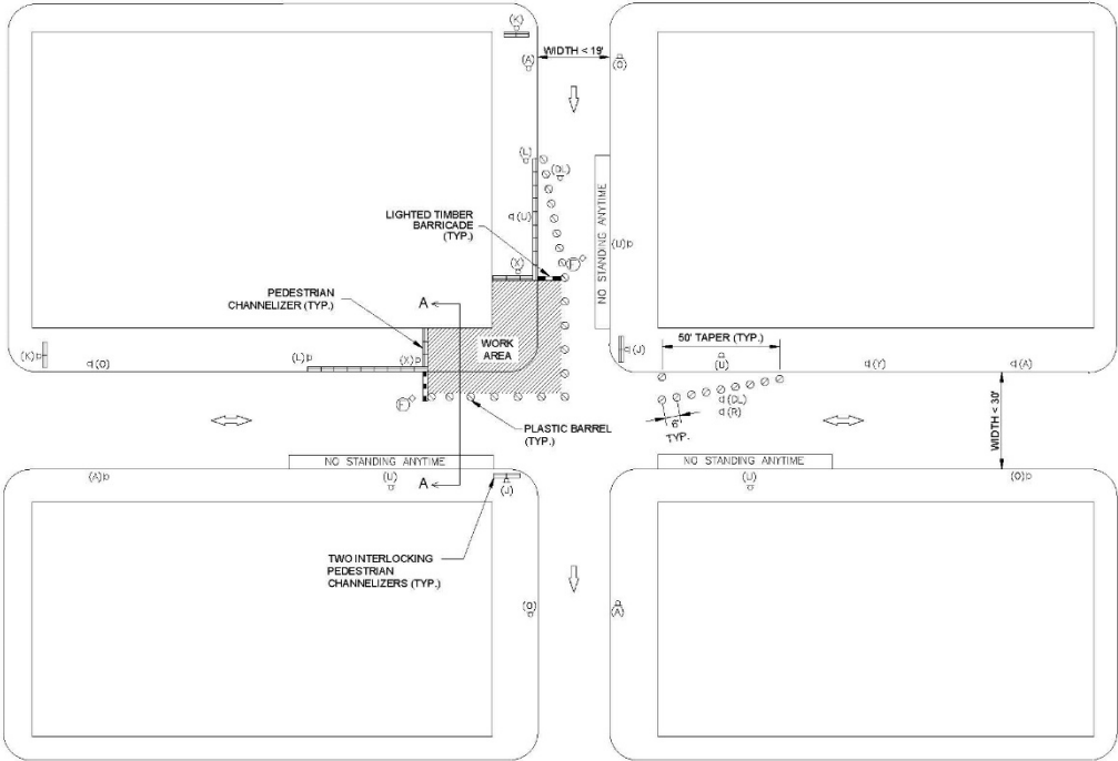
TYPICAL PLAN NOT TO SCALE
