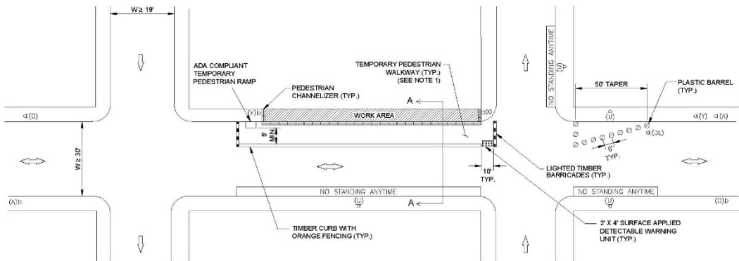
TYPICAL PLAN NOT TO SCALE
