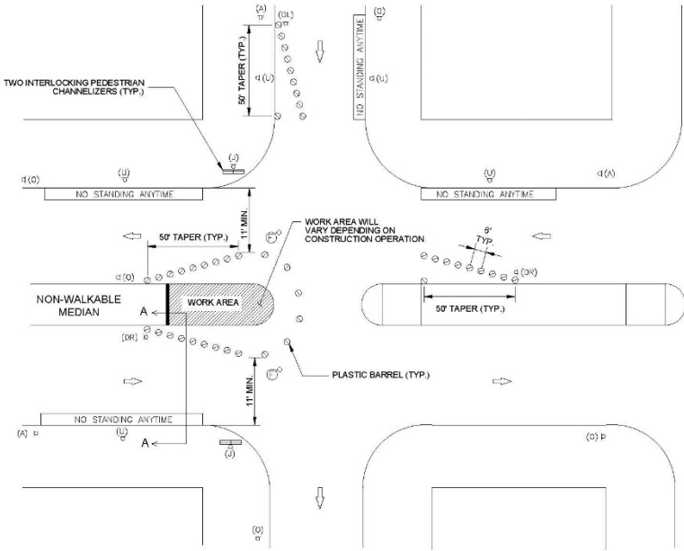
TYPICAL PLAN NOT TO SCALE
