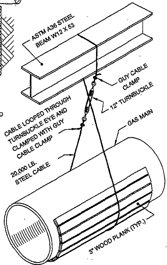
DETAIL "B"
