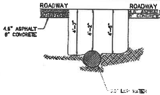
SECTION LOOKING SOUTHWEST
