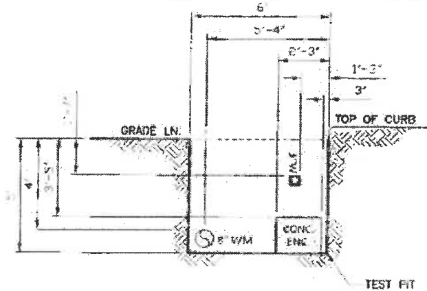
PROFILE — LOOKING NORTH N.T.S.
