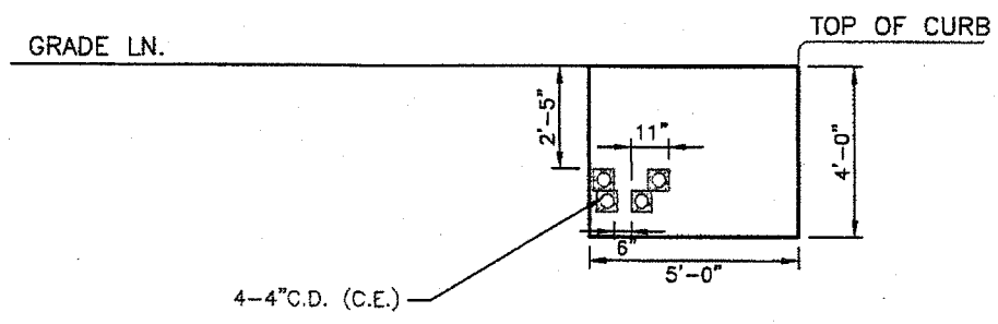
PROFILE - LOOKING NORTH N.T.S.
