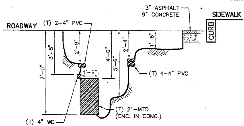
SECTION LOOKING WEST
