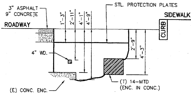
SECTION LOOKING NORTH
