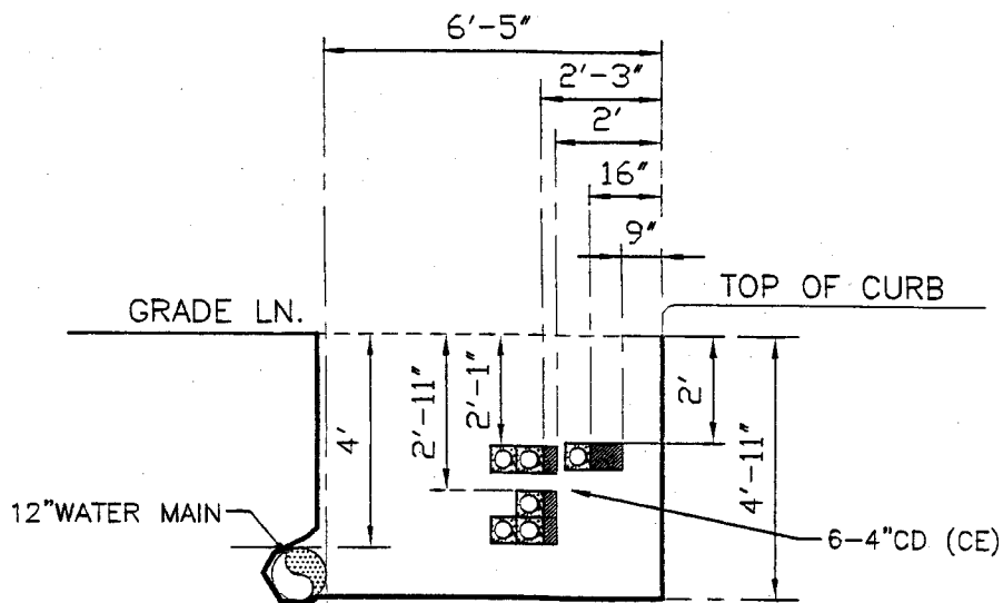
PROFILE - LOOKING NORTH N.T.S.
