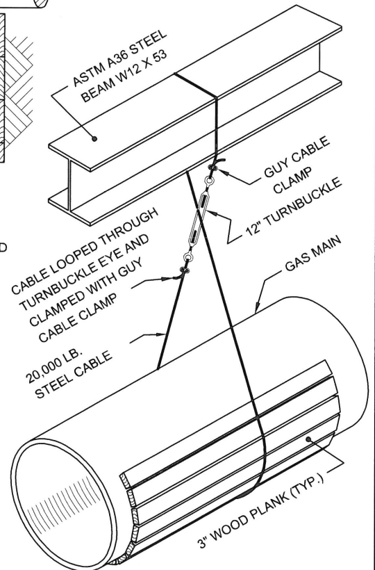
DETAIL "B"
