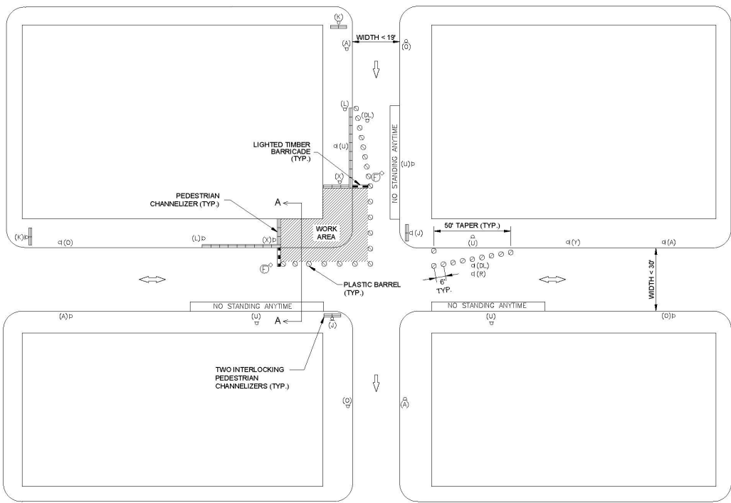
TYPICAL PLAN NOT TO SCALE
