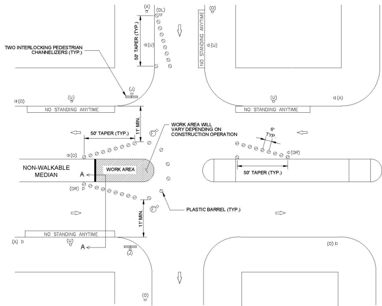
TYPICAL PLAN NOT TO SCALE
