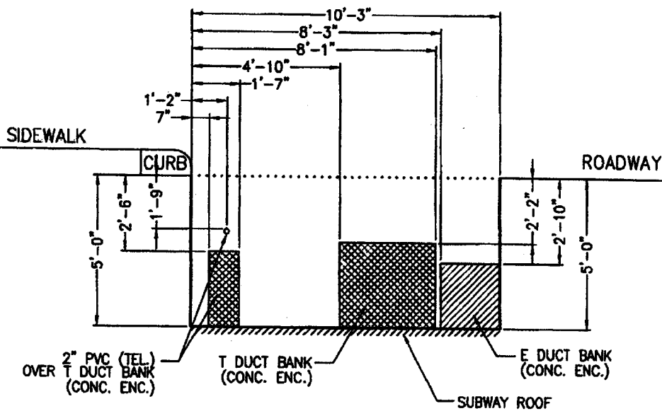
SECTION LOOKING NORTH
