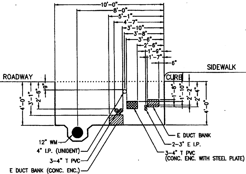
SECTION LOOKING SOUTH
