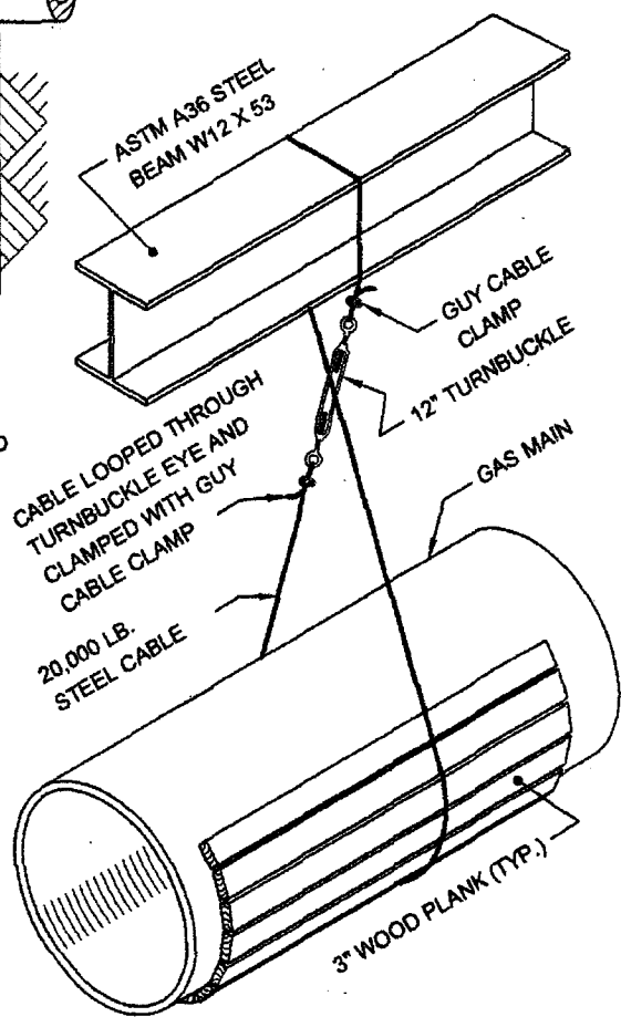
DETAIL "B"
