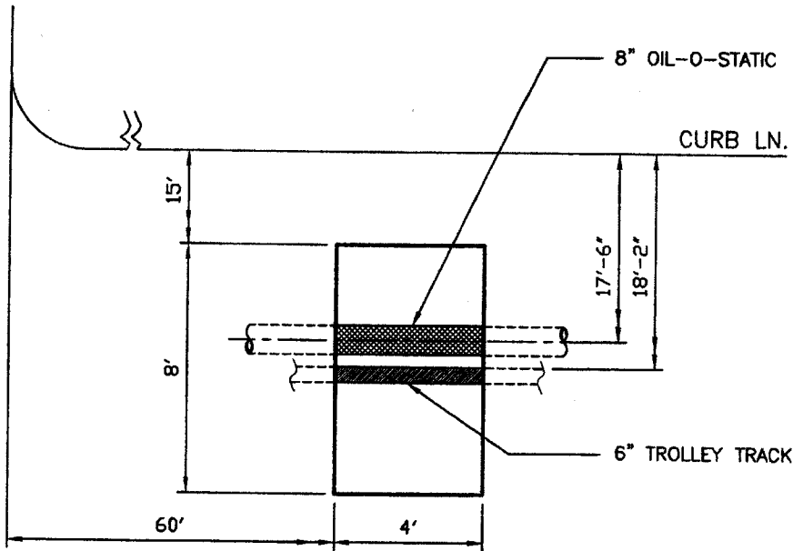
FULTON ST. PLAN
