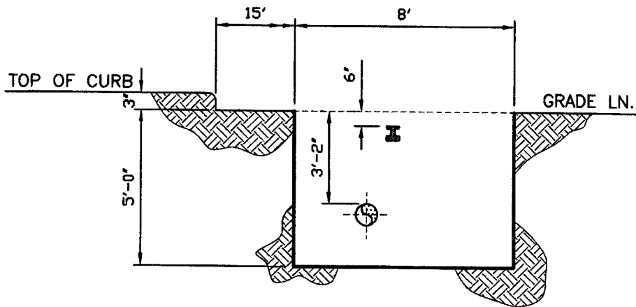
PROFILE - LOOKING EAST
